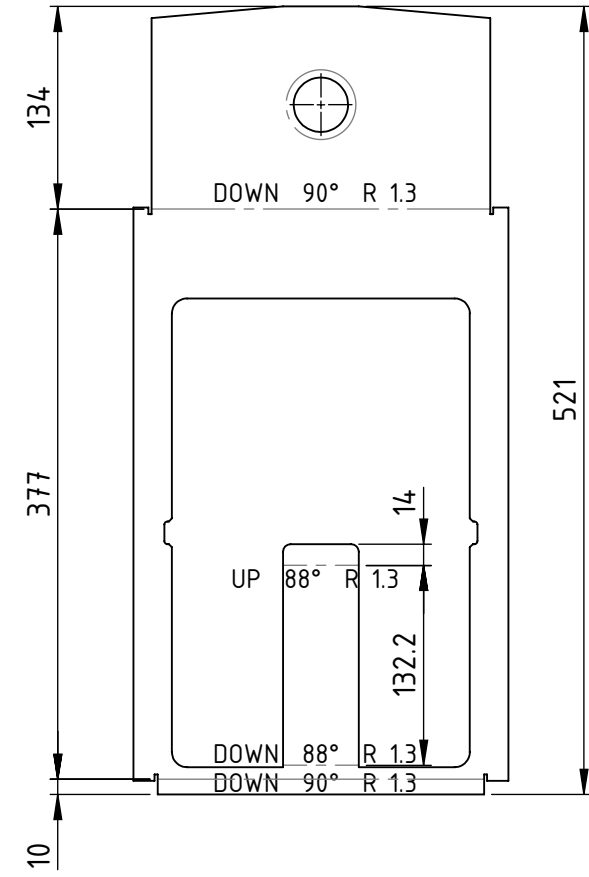
FLAT PATTERN VIEW
